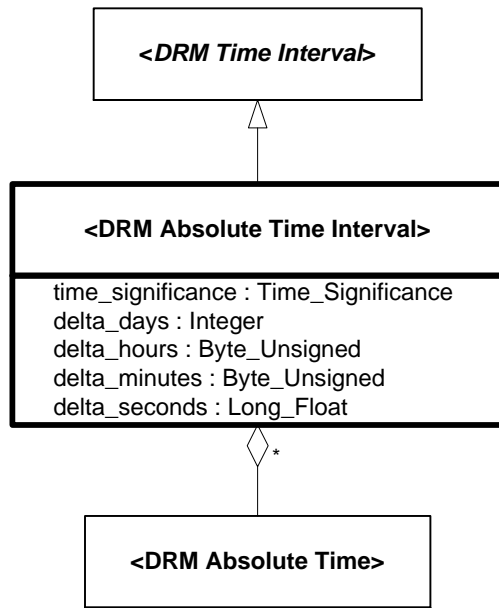
Figure 6.2 — DRM_Absolute_Time_Interval
