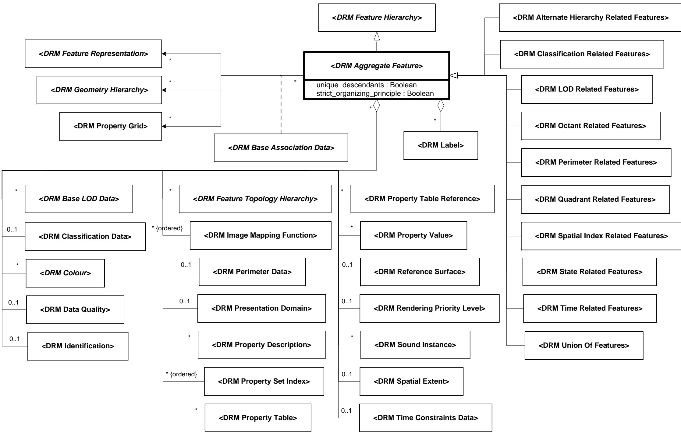
Figure 6.3 — DRM_Aggregate_Feature
