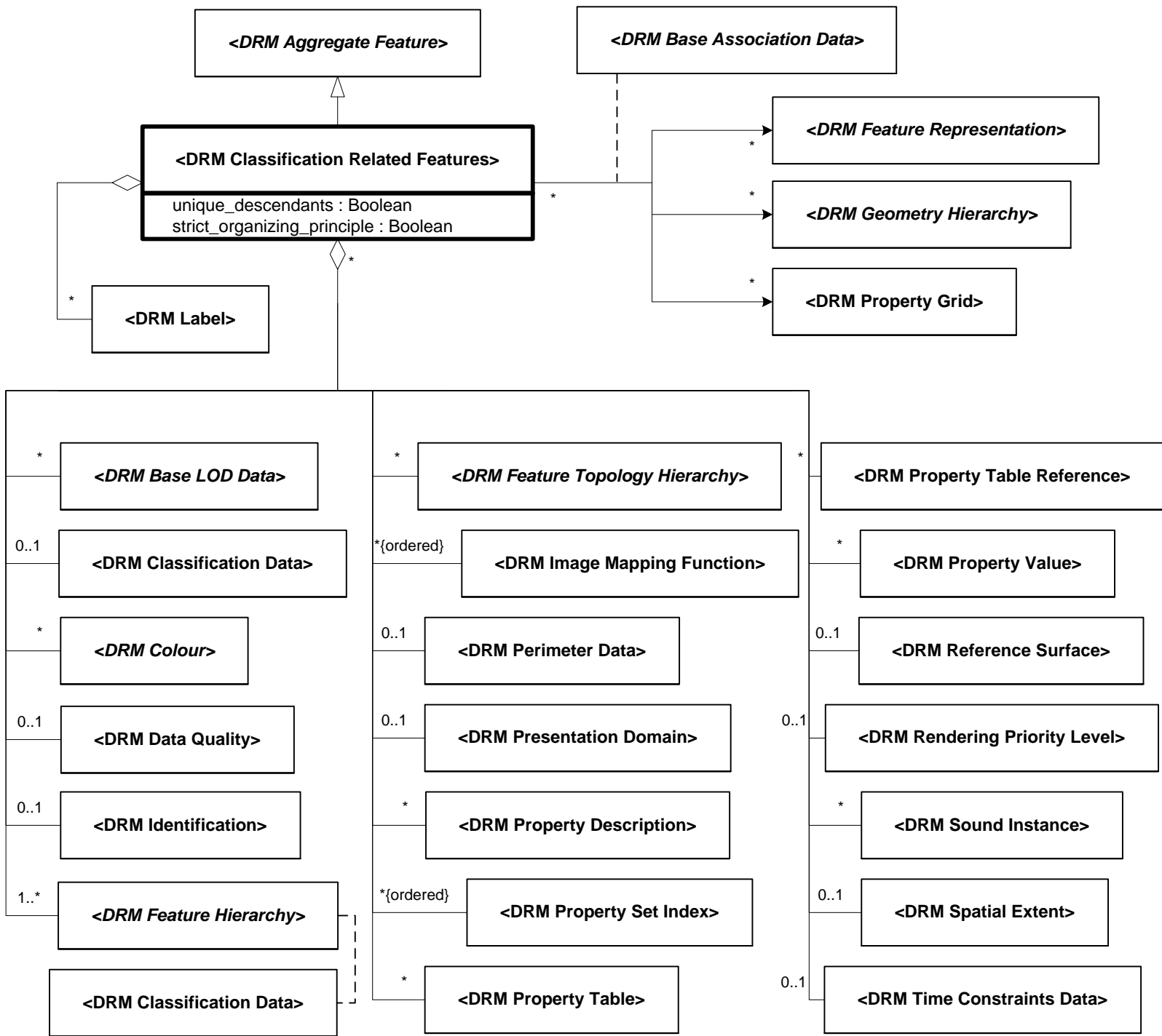
Figure 6.32 — DRM_Classification_Related_Features
