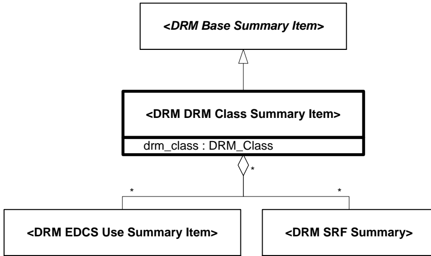
Figure 6.66 — DRM_DRM_Class_Summary_Item
