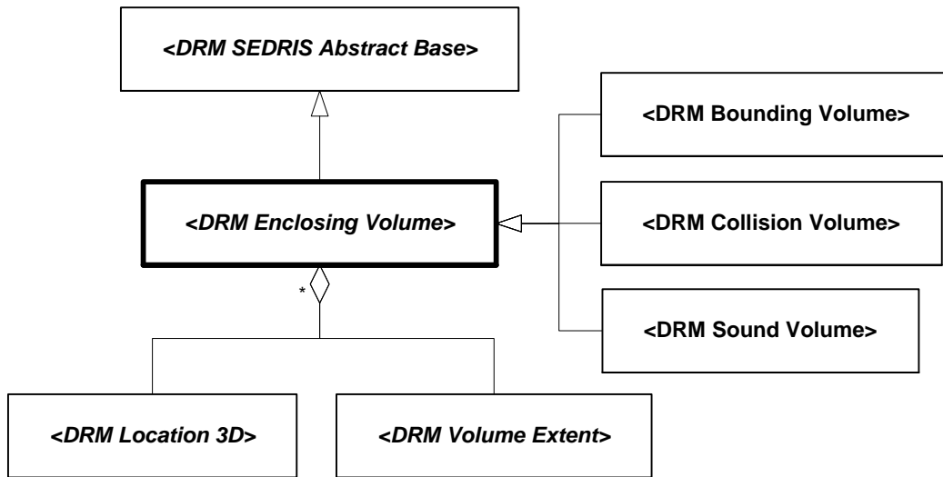
Figure 6.78 — DRM_Enclosing_Volume
