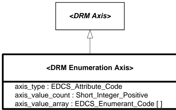
Figure 6.79 — DRM_Enumeration_Axis
