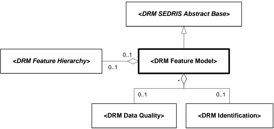
Figure 6.90 — DRM_Feature_Model
