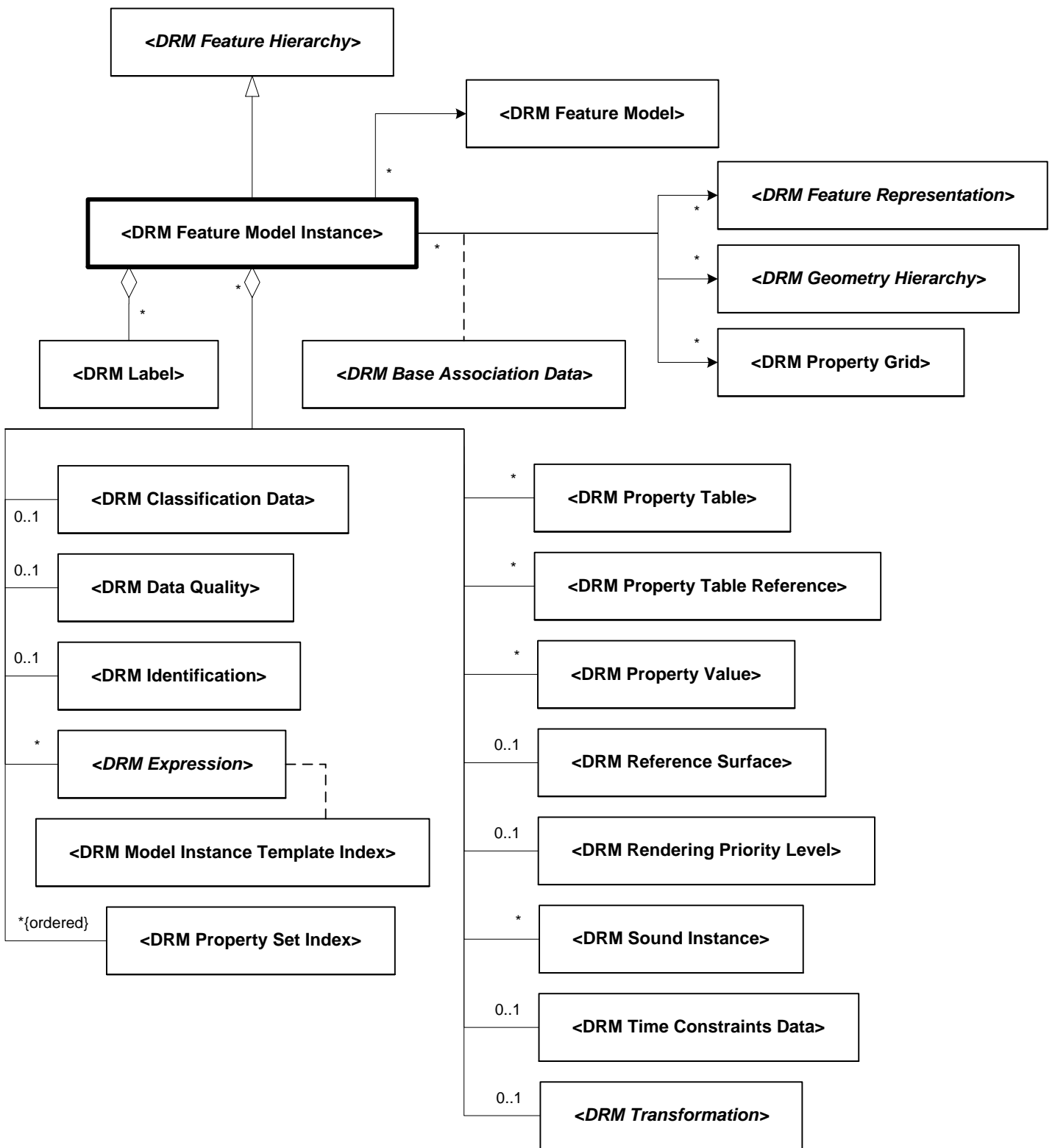
Figure 6.91 — DRM_Feature_Model_Instance
