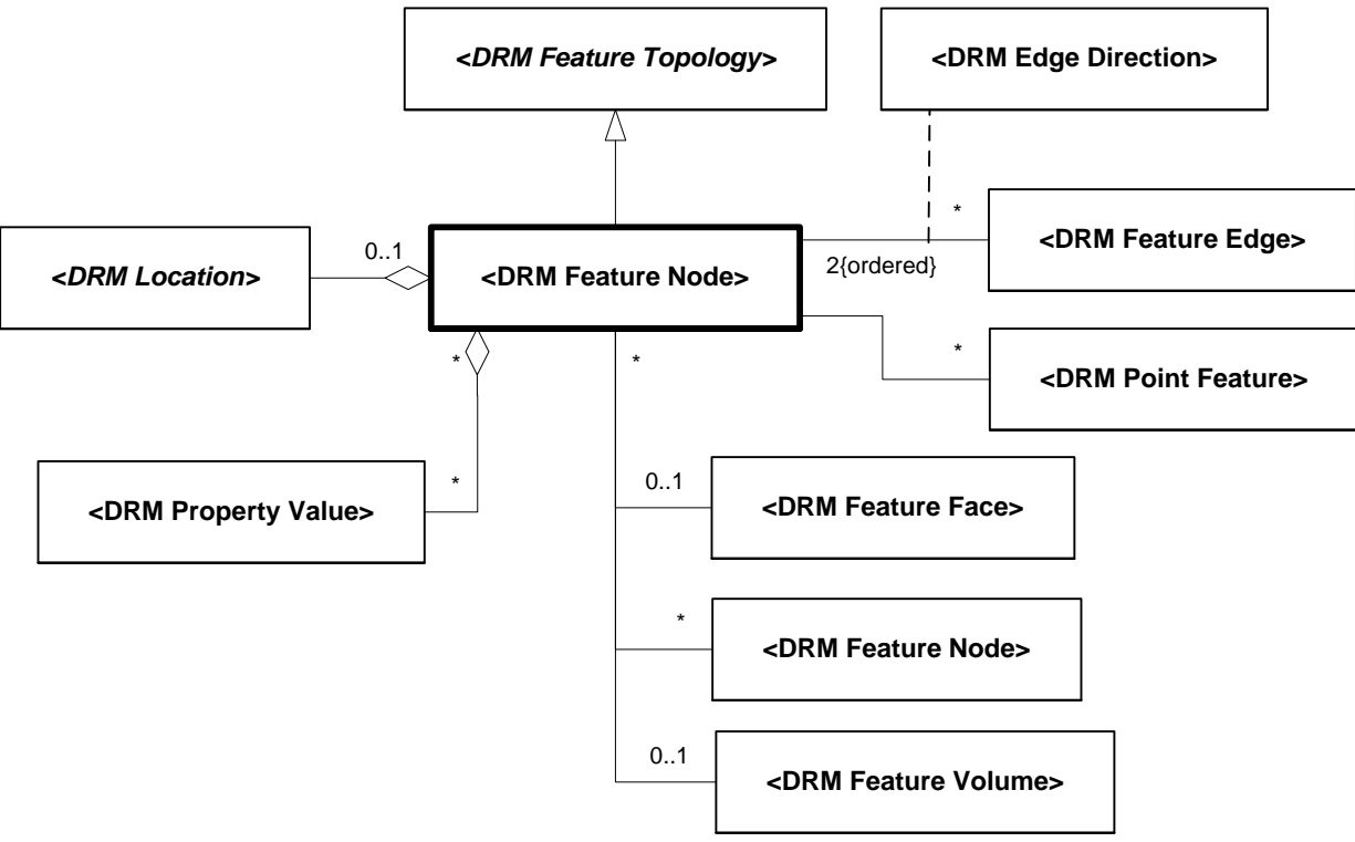
Figure 6.92 — DRM_Feature_Node
