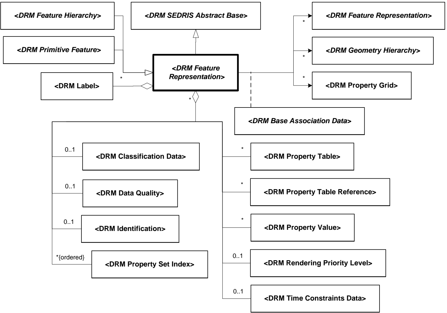
Figure 6.93 — DRM_Feature_Representation
