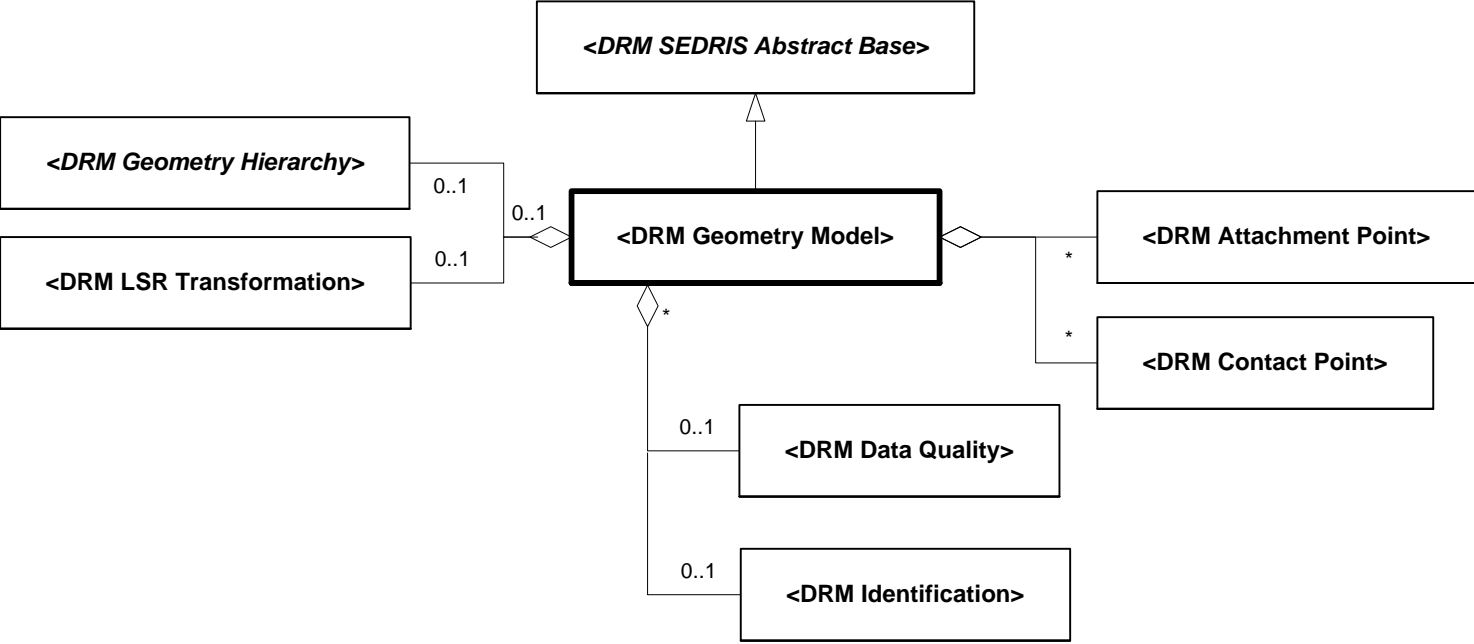
Figure 6.110 — DRM_Geometry_Model
