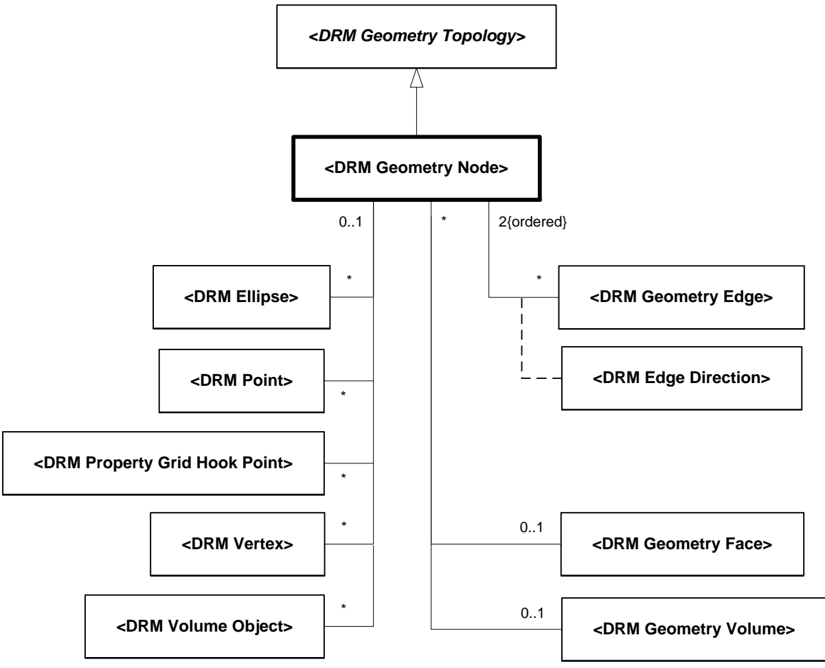
Figure 6.112 — DRM_Geometry_Node
