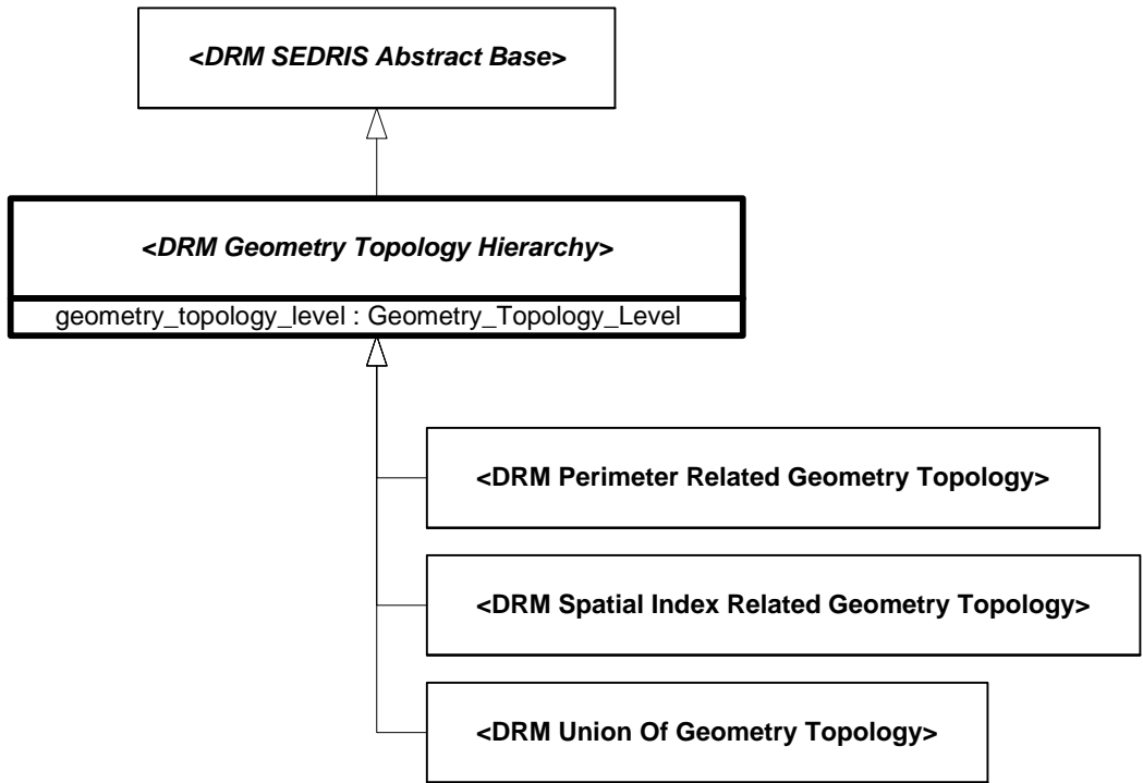
Figure 6.115 — DRM_Geometry_Topology_Hierarchy
