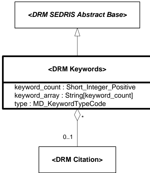
Figure 6.144 — DRM_Keywords
