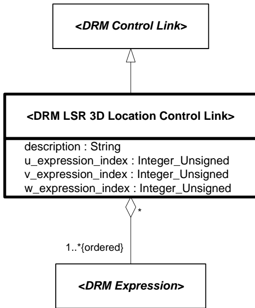
Figure 6.178 — DRM_LSR_3D_Location_Control_Link
