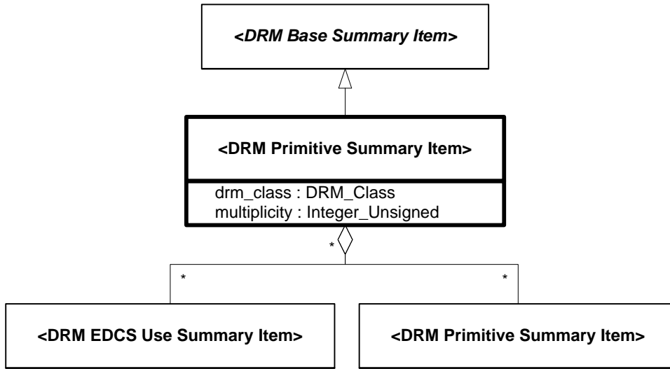
Figure 6.227 — DRM_Primitive_Summary_Item
