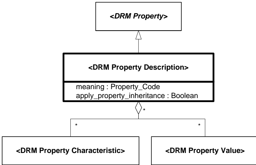
Figure 6.232 — DRM_Property_Description
