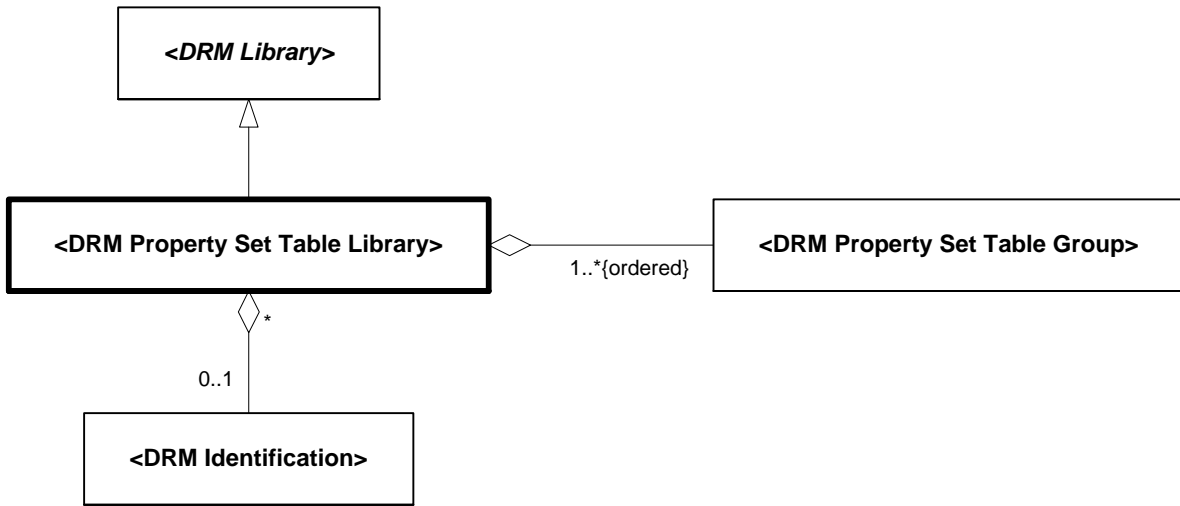
Figure 6.243 — DRM_Property_Set_Table_Library
