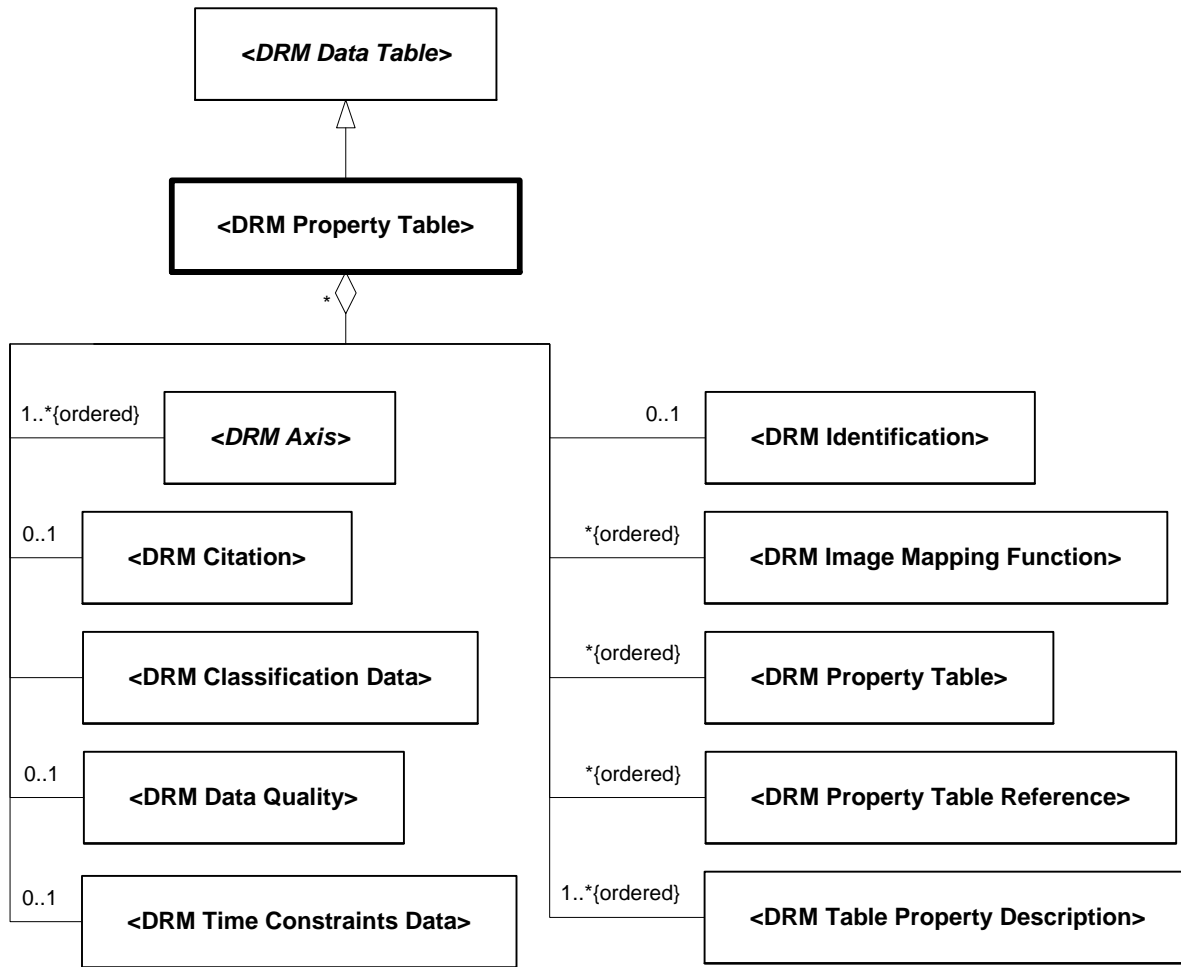
Figure 6.244 — DRM_Property_Table
