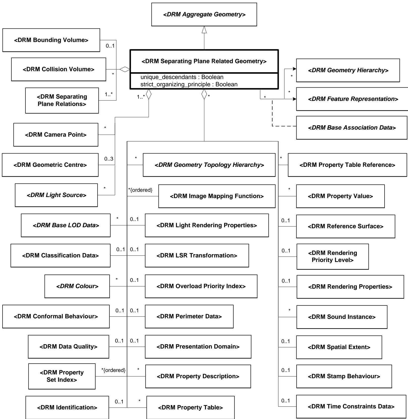
Figure 6.295 — DRM_Separating_Plane_Related_Geometry
