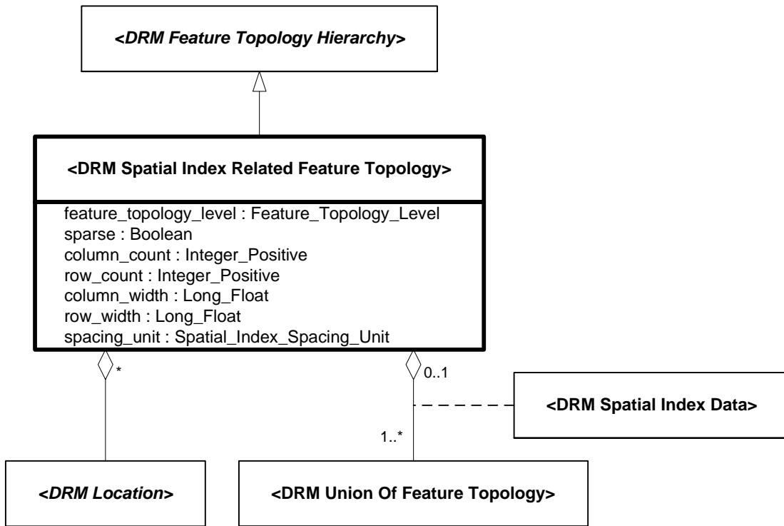
Figure 6.310 — DRM_Spatial_Index_Related_Feature_Topology
