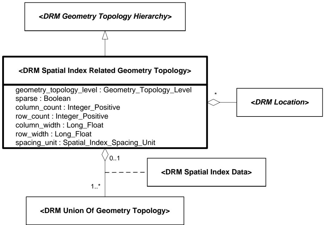
Figure 6.318 — DRM_Spatial_Index_Related_Geometry_Topology
