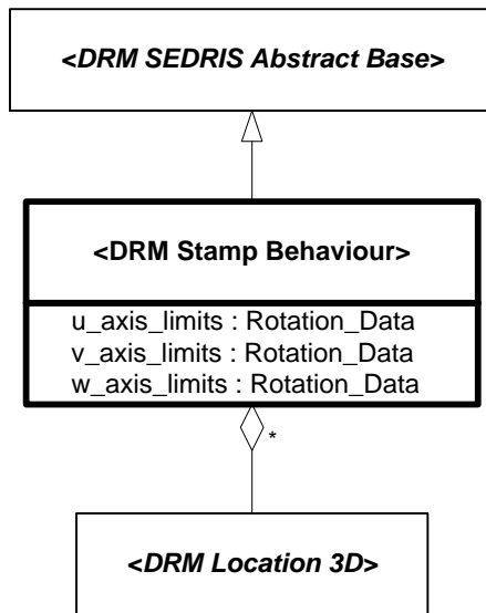
Figure 6.325 — DRM_Stamp_Behaviour
