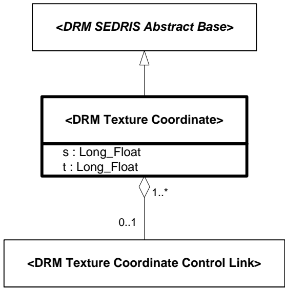
Figure 6.342 — DRM_Texture_Coordinate
