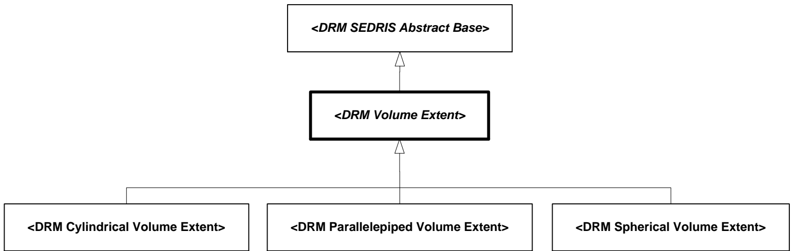
Figure 6.372 — DRM_Volume_Extent
