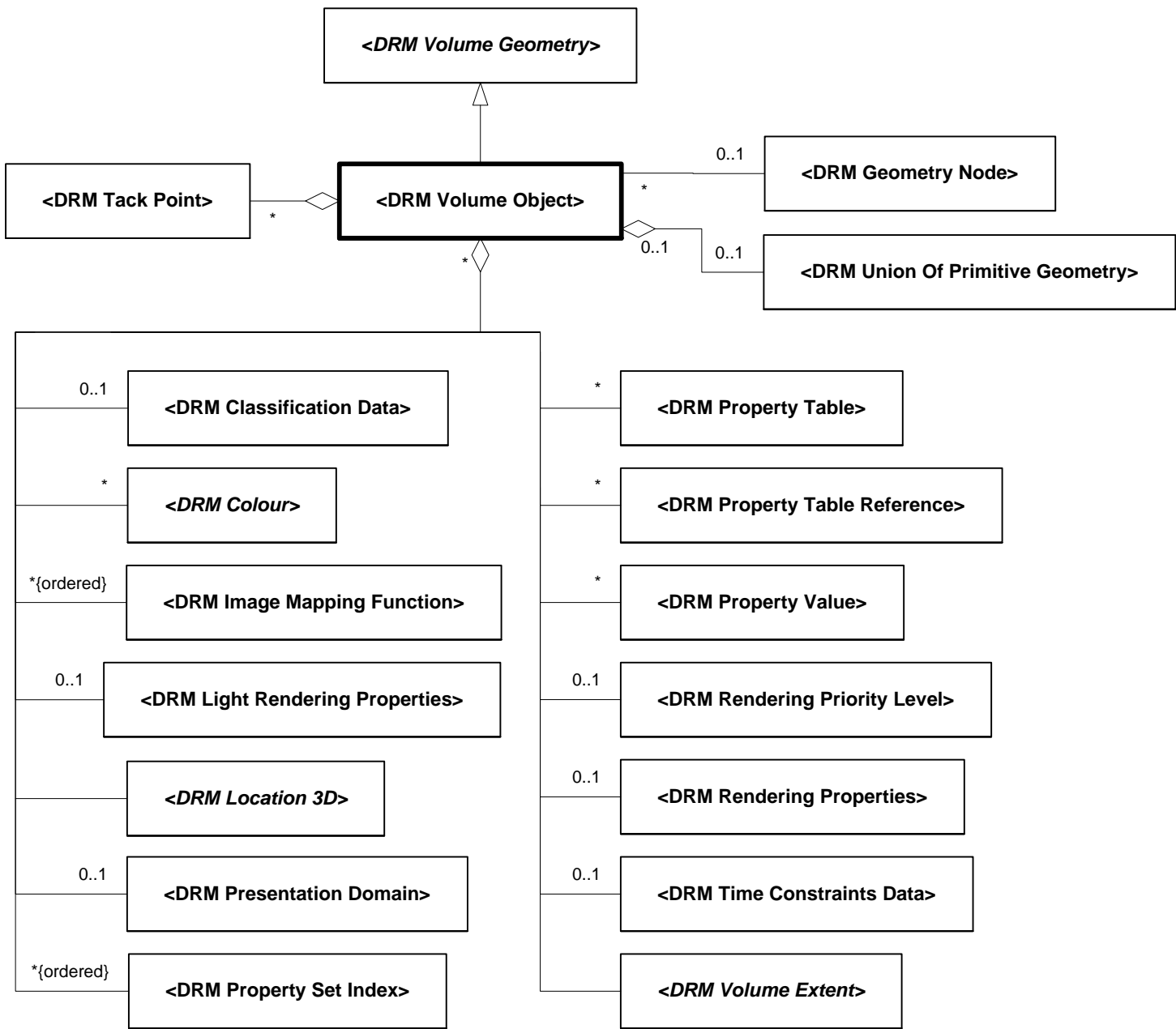
Figure 6.377 — DRM_Volume_Object
