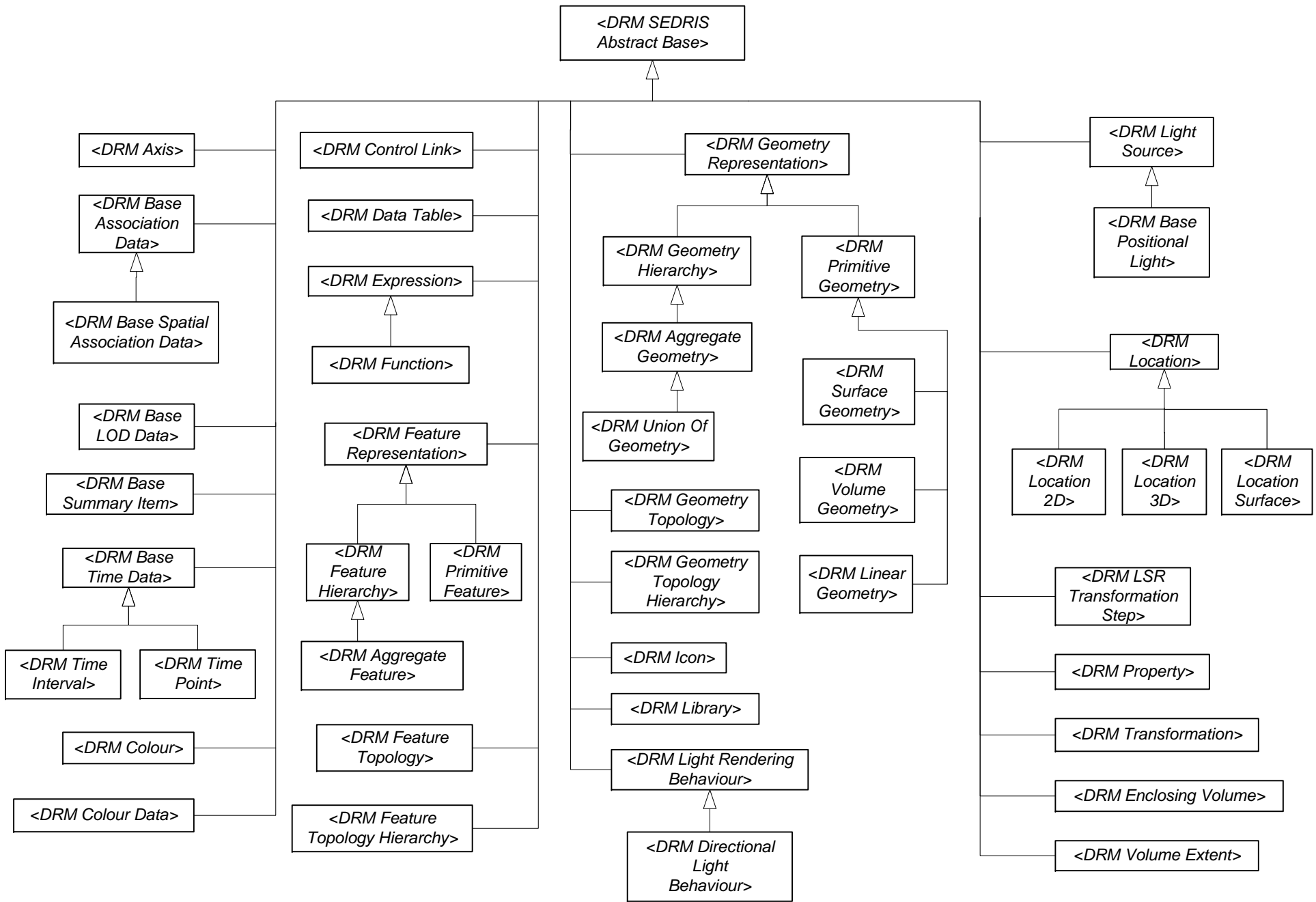
Figure A.24 — Abstract class hierarchy
