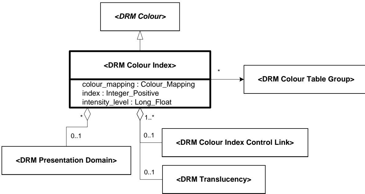
Figure 6.41 — DRM_Colour_Index
