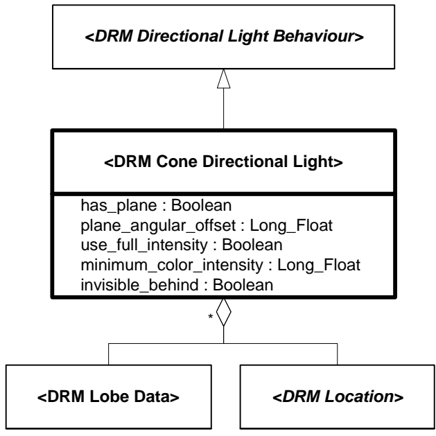
Figure 6.48 — DRM_Cone_Directional_Light
