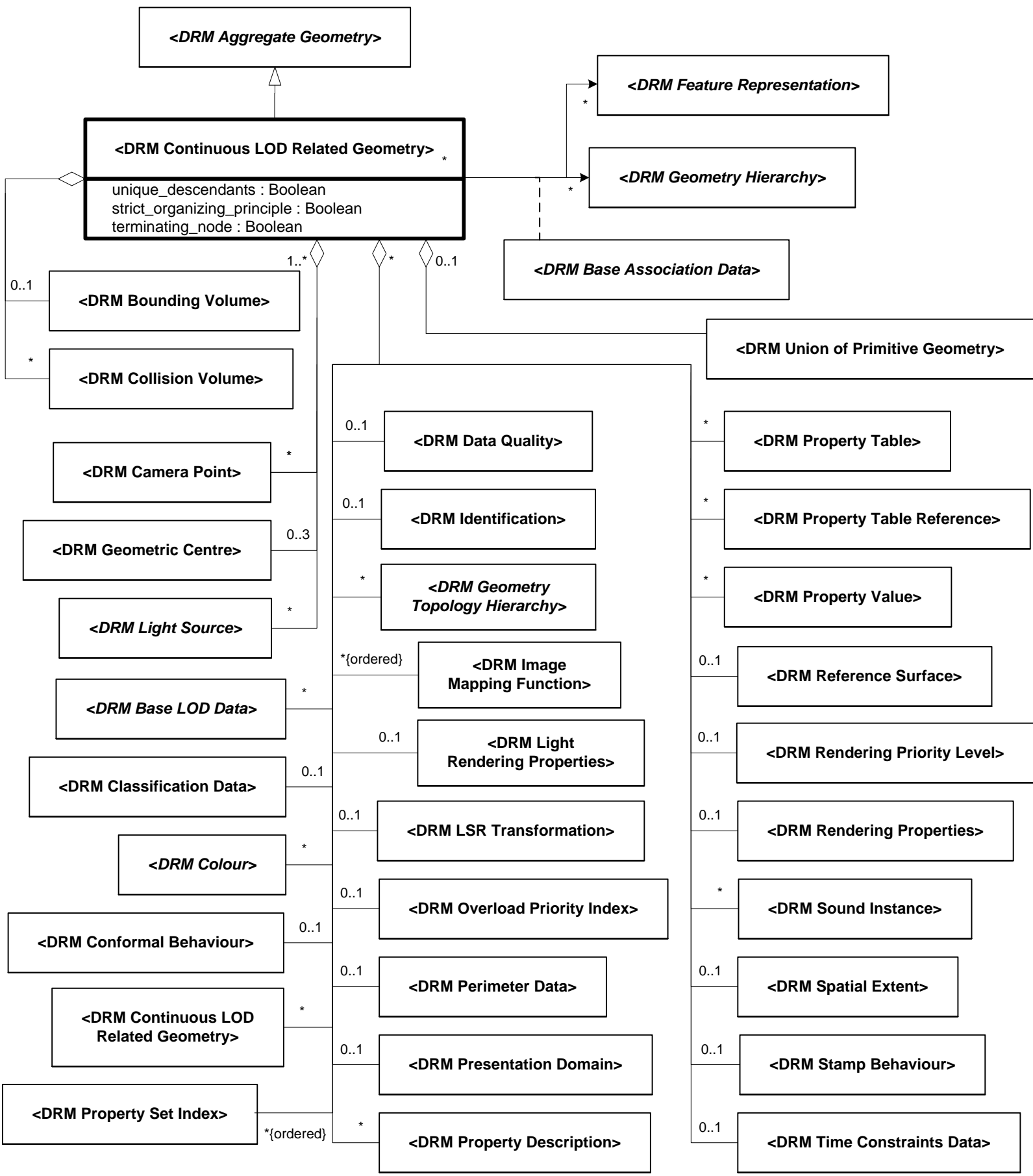
Figure 6.55 — DRM_Continuous_LOD_Related_Geometry
