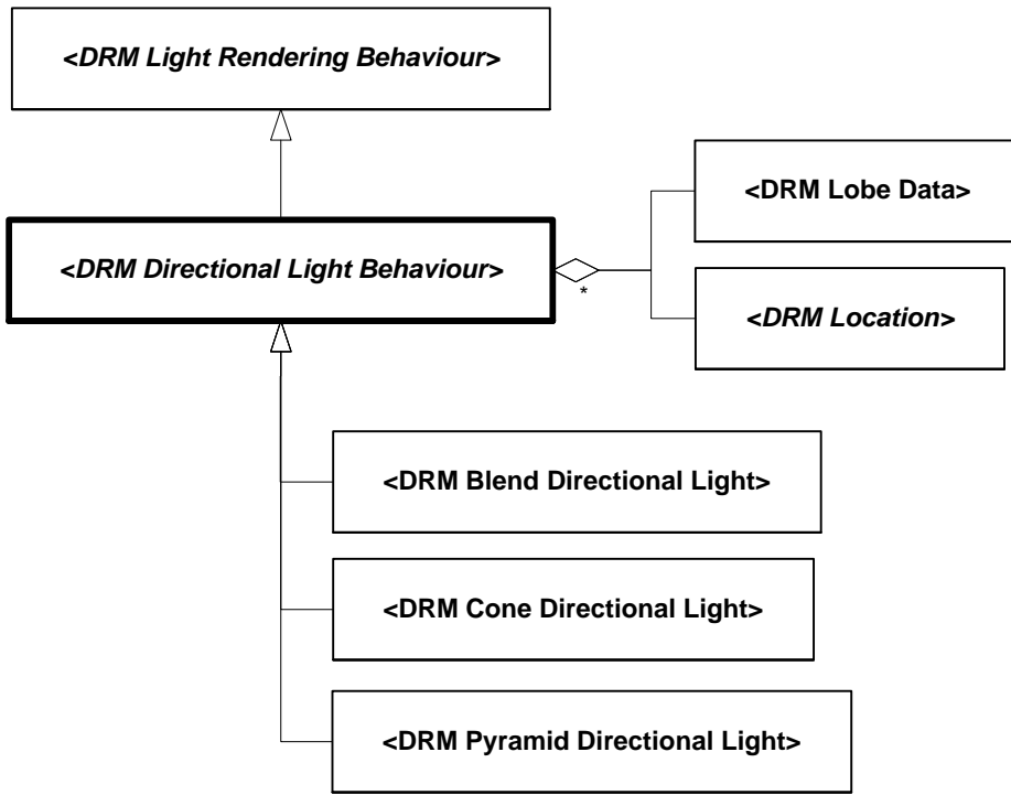
Figure 6.63 — DRM_Directional_Light_Behaviour
