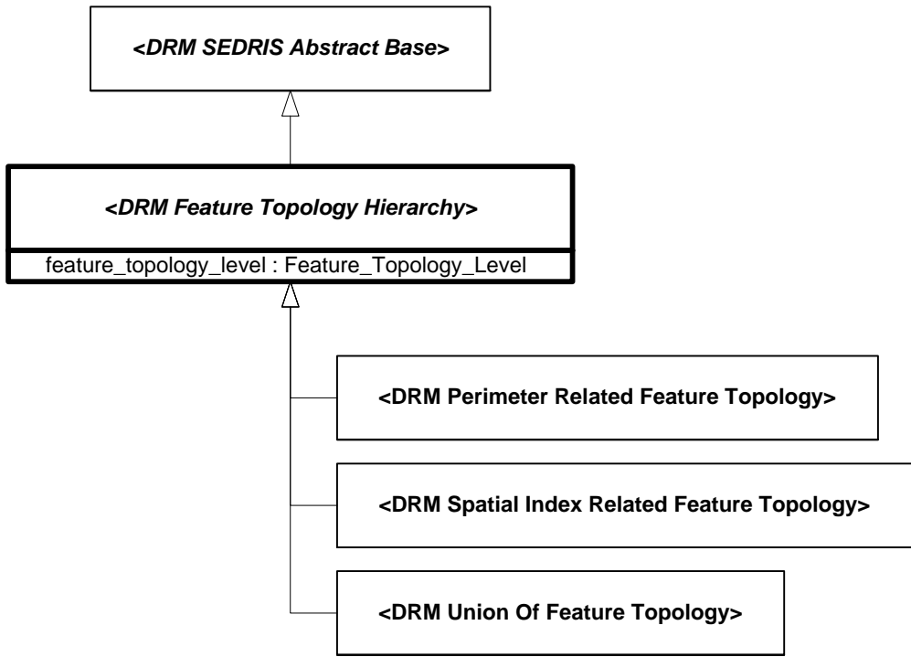
Figure 6.95 — DRM_Feature_Topology_Hierarchy
