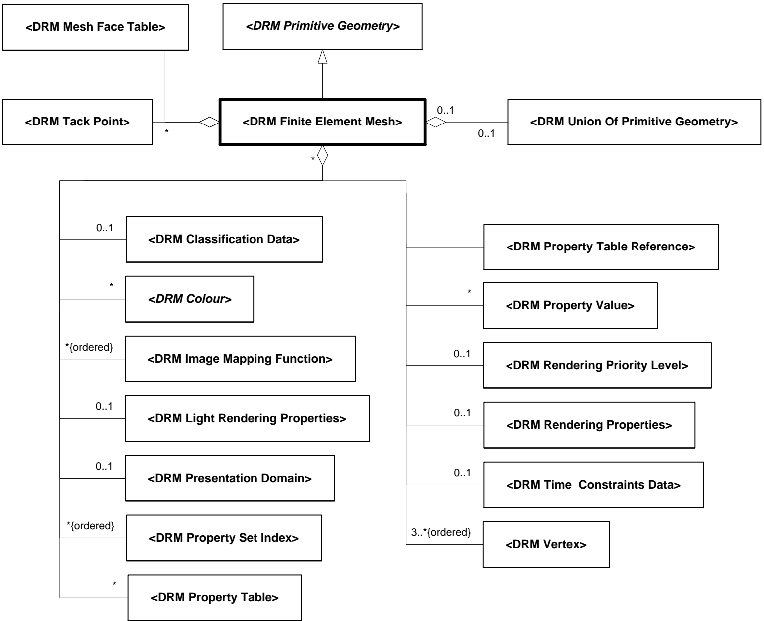
Figure 6.99 — DRM_Finite_Element_Mesh
