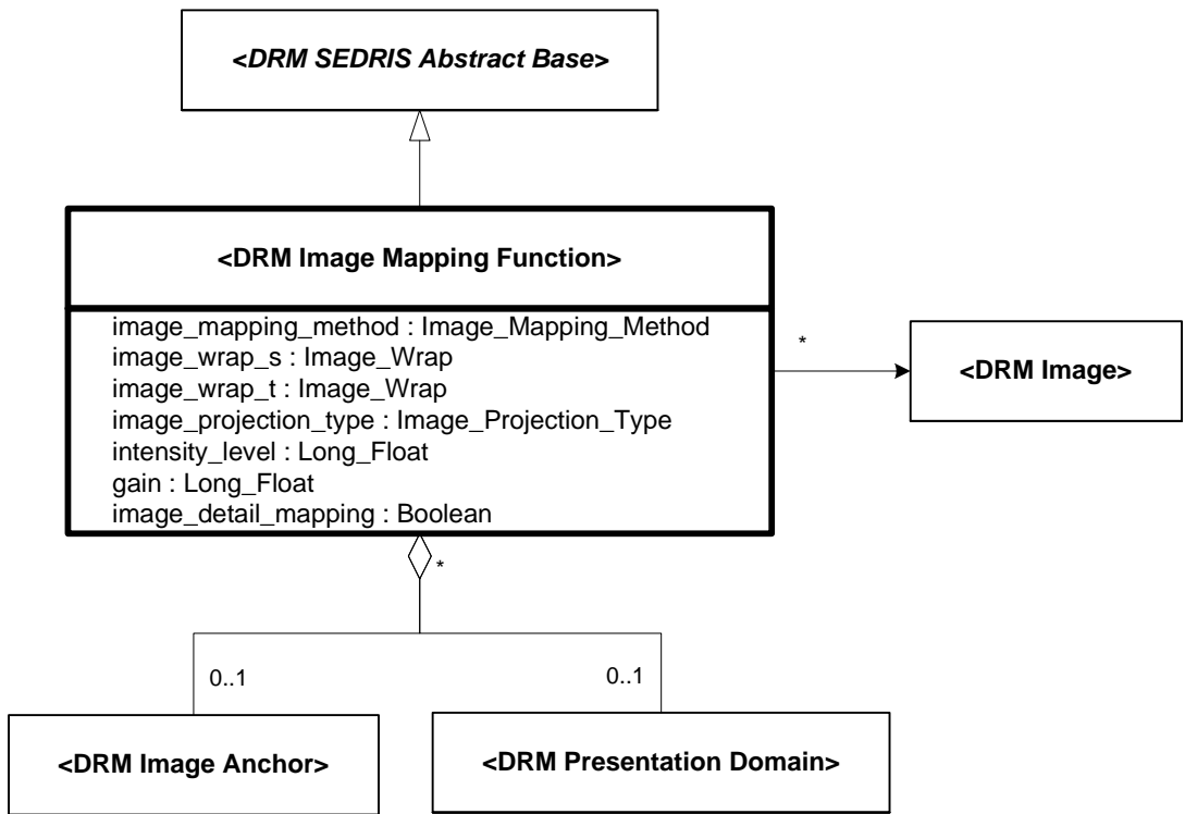
Figure 6.134 — DRM_Image_Mapping_Function
