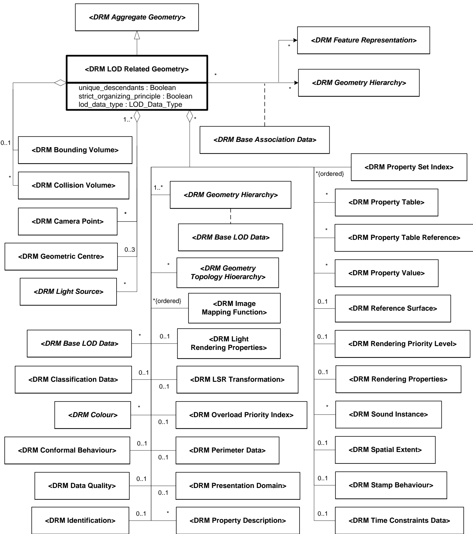
Figure 6.171 — DRM_LOD_Related_Geometry
