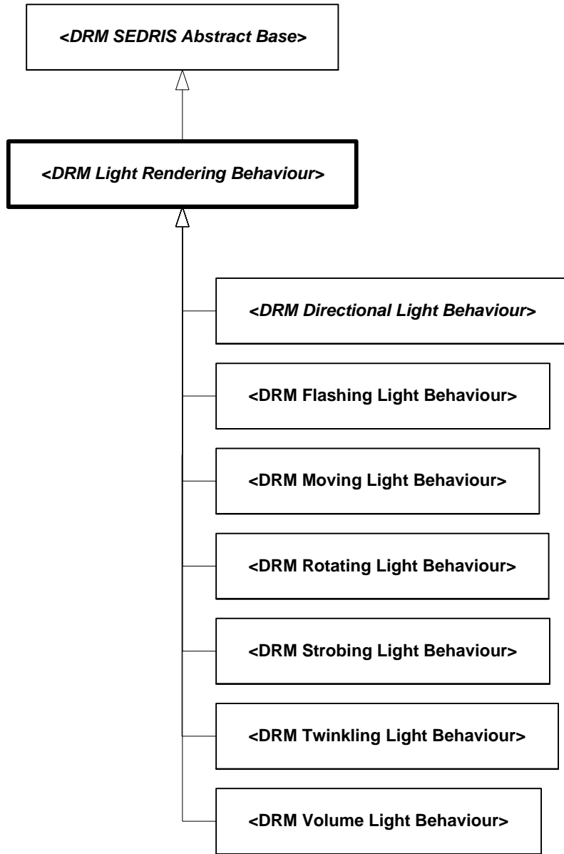
Figure 6.151 — DRM_Light_Rendering_Behaviour
