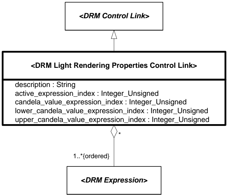
Figure 6.153 — DRM_Light_Rendering_Properties_Control_Link
