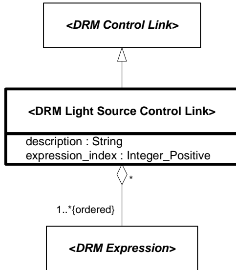
Figure 6.155 — DRM_Light_Source_Control_Link
