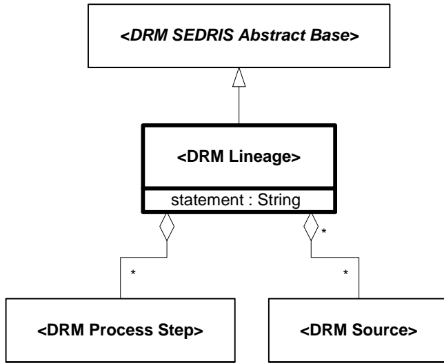
Figure 6.157 — DRM_Lineage
