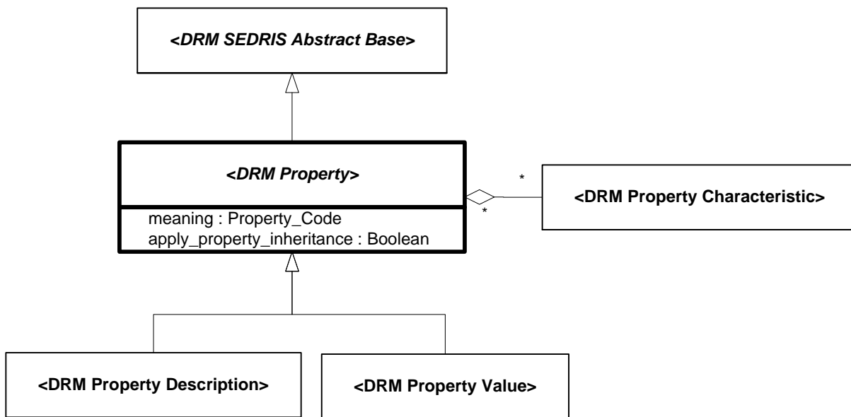
Figure 6.230 — DRM_Property
