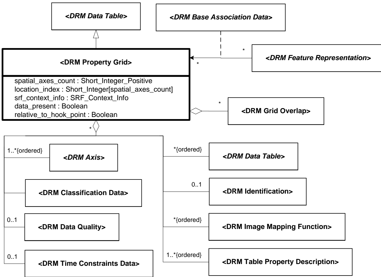
Figure 6.235 — DRM_Property_Grid
