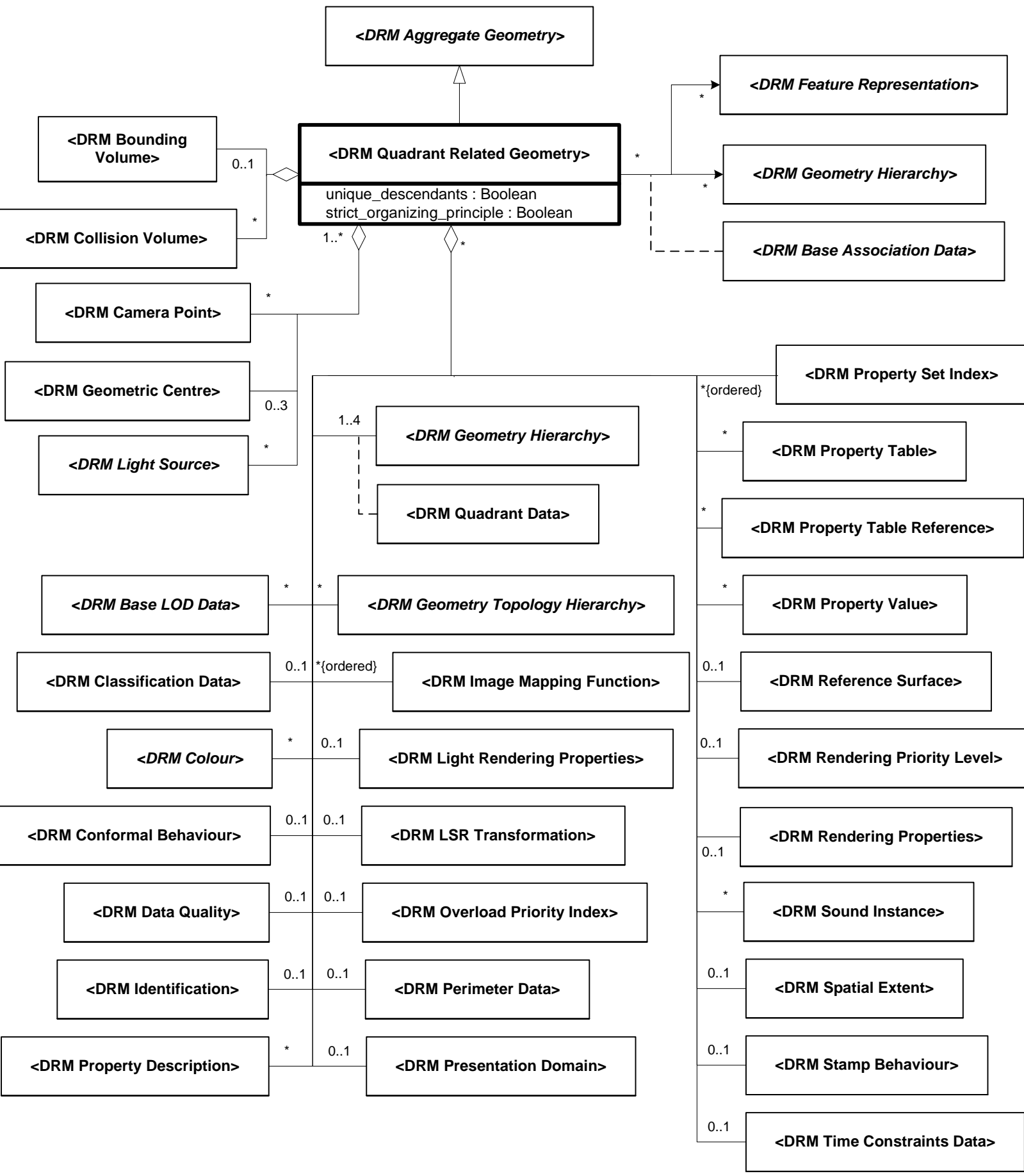
Figure 6.262 — DRM_Quadrant_Related_Geometry
