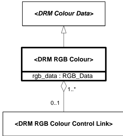
Figure 6.280 — DRM_RGB_Colour
