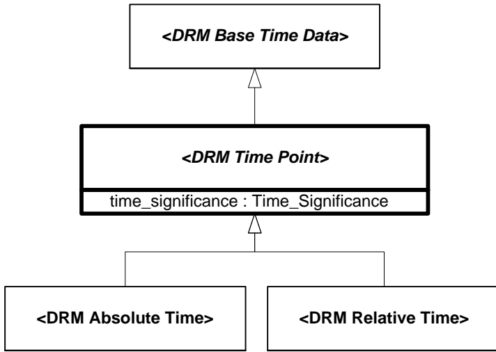
Figure 6.347 — DRM_Time_Point
