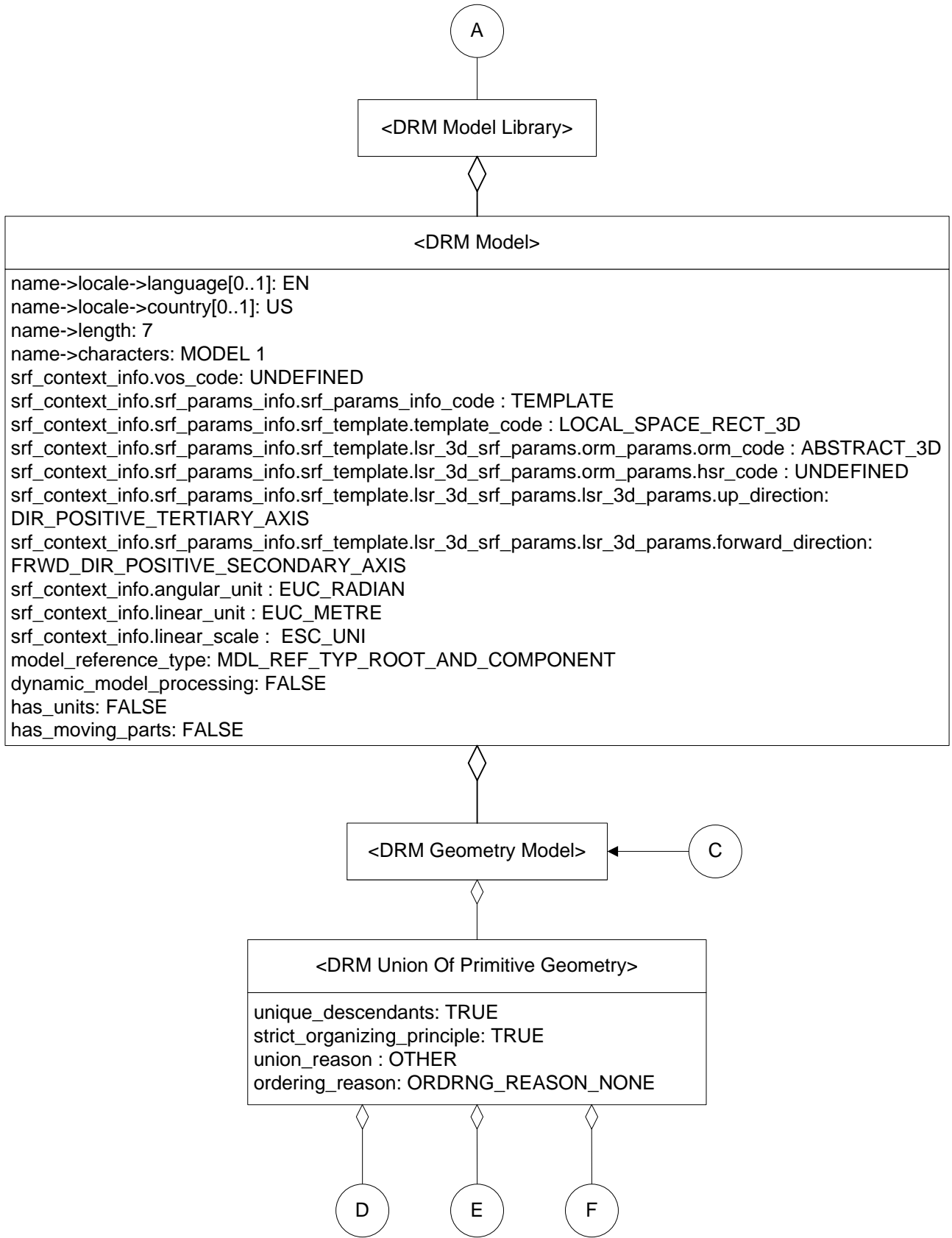
Figure B.3 – DRM model instantiated within the DRM environment root
