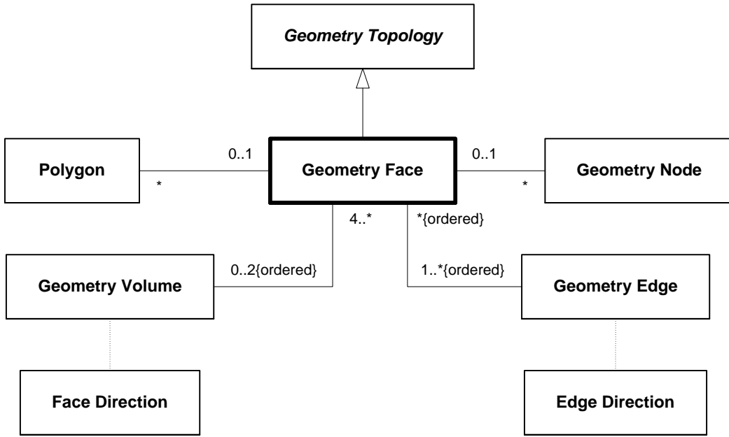
Figure 6.108 — DRM_Geometry_Face
