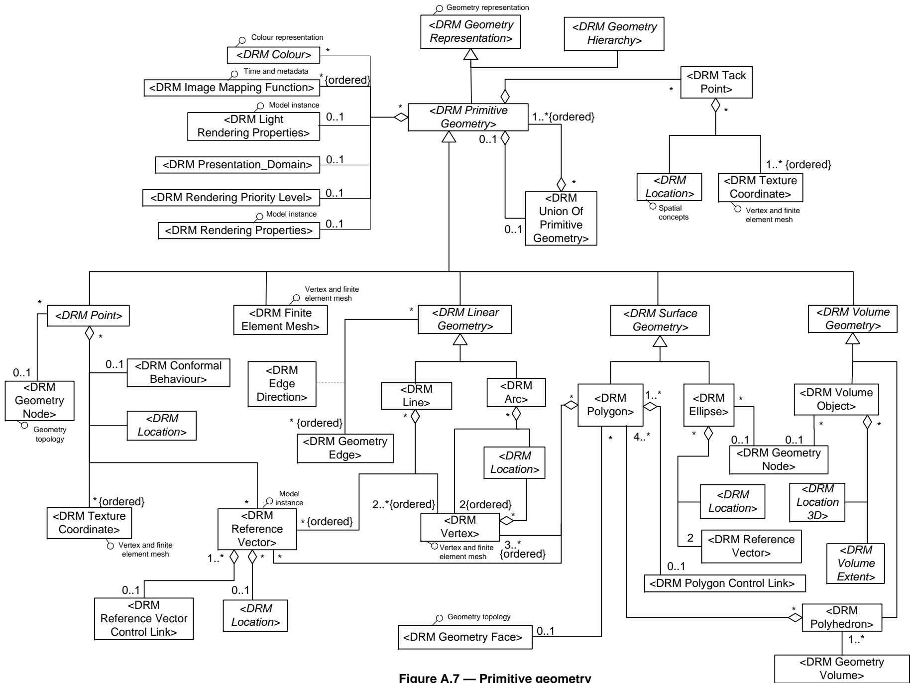
Figure A.7 — Primitive geometry
